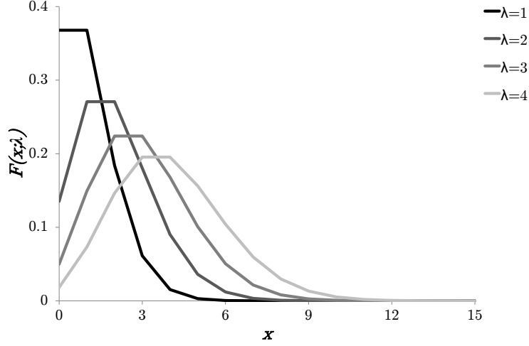
Figure 3: Poisson distributions for various measured and expected occurrences, i.e., x and \lambda , respectively
